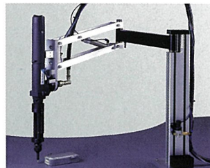
7535 Pantograph workstation
